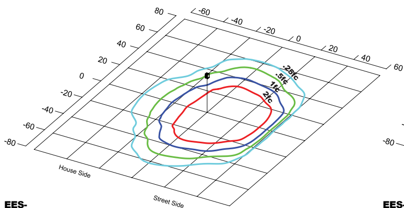
EES- KH25C1X112UKG C Type III Grid in MH MH=20 Feet
