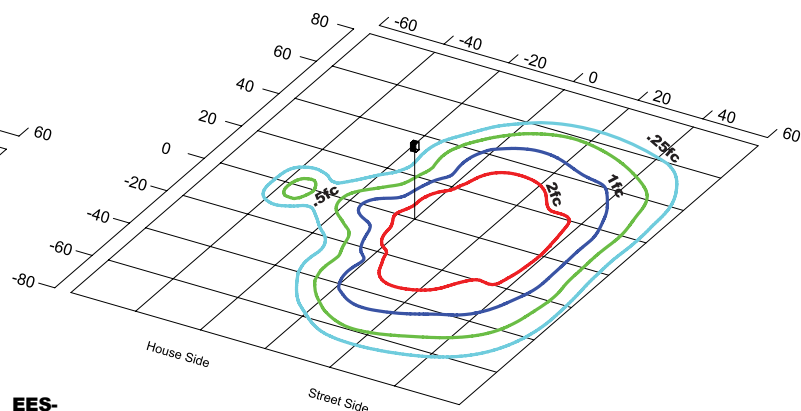
EES- KH25D1X112UKG C Type IV Grid in MH MH=20 Feet
