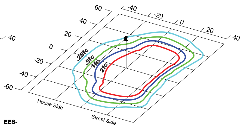
EES- KH25Q1X112UKG C Type II Grid in MH MH=20 Feet
