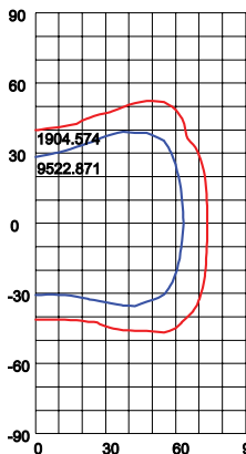
"A" = NEMA 7H x 5V 256W Max. Candela = 34,471
