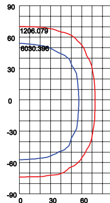
"F" = NEMA 7H x 7V 256W Max. Candela = 34,459
