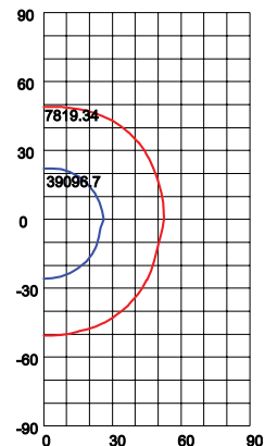
"I" = NEMA 4H x 4V 293W Max. Candela = 37,035
