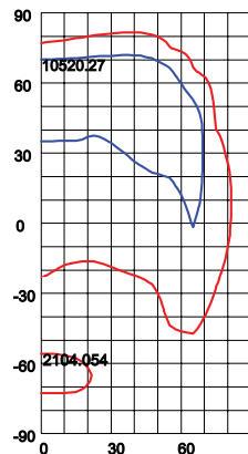
"D" = NEMA 7H x 6V 256W Max. Candela = 34,221
