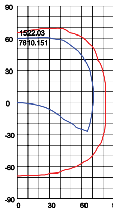
"C" = NEMA 7H x 7V 256W Max. Candela = 36,926
